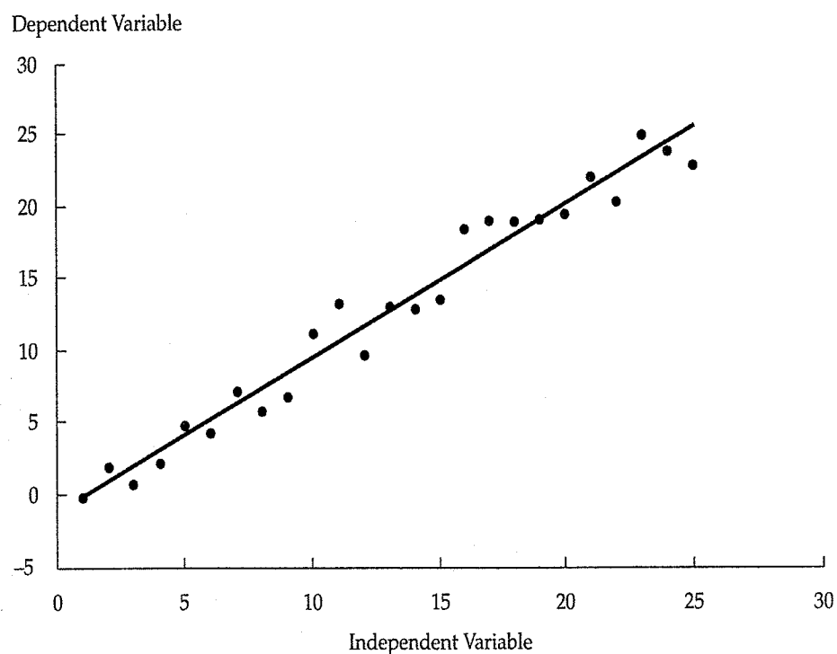
FIGURE 9-1 Regression with Homoskedasticity
