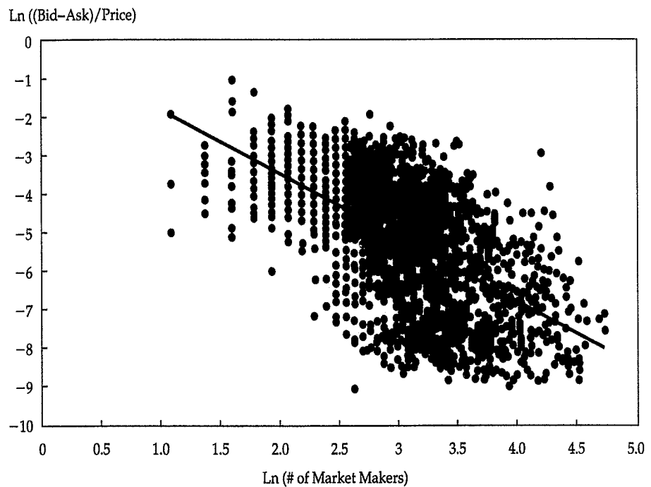
FIGURE 9-4 Linear Regression When Two Variables Have a Linear Relation
