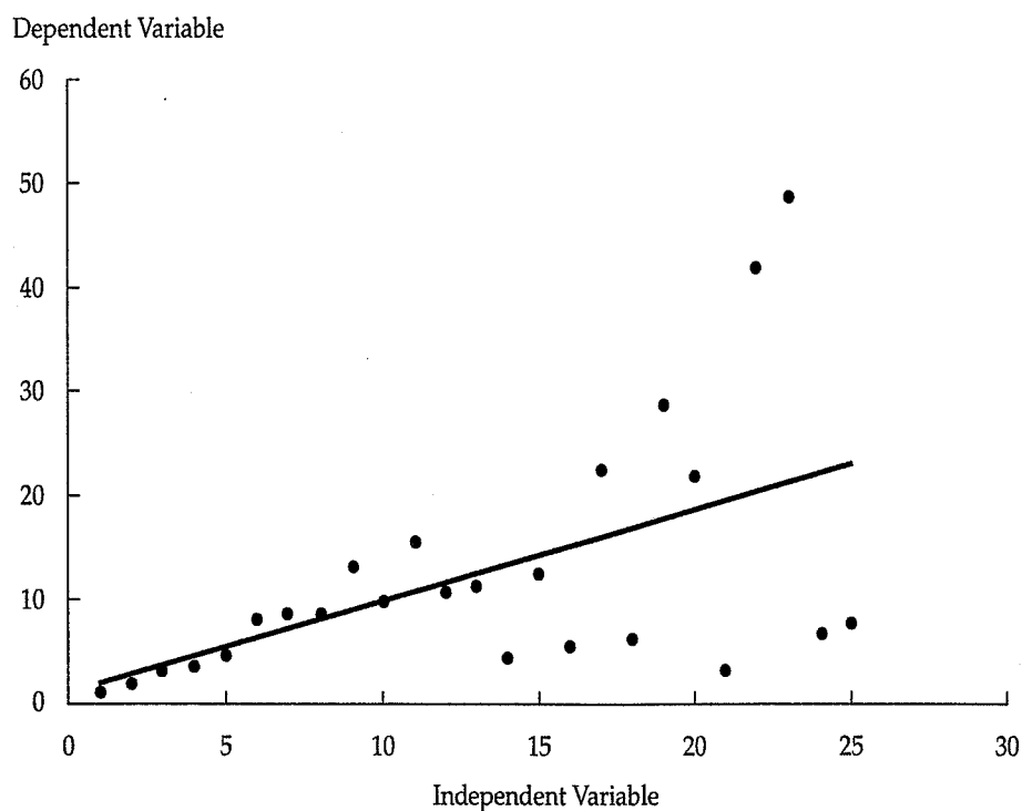
FIGURE 9-2 Regression with Heteroskedasticity
