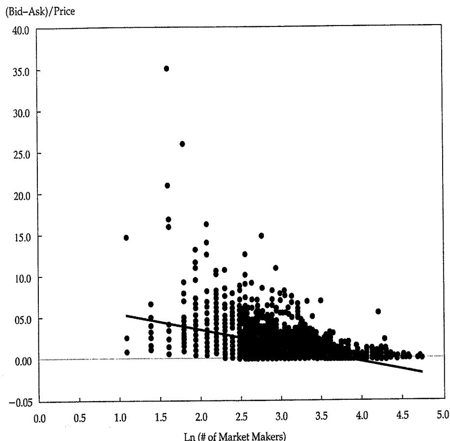
FIGURE 9-5 Linear Regression When Two Variables Have a Nonlinear Relation
